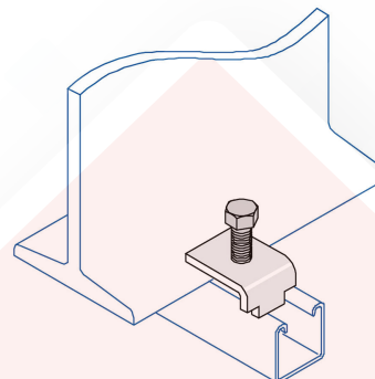
Steel Beam Holder post
